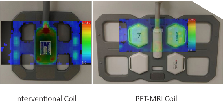
Fig. 1- Color-coded map of the planar PET attenuation factor overlaid onto a photographic image of the interventional DuoFLEX coil and the standard PET-MRI flexible surface coil.
