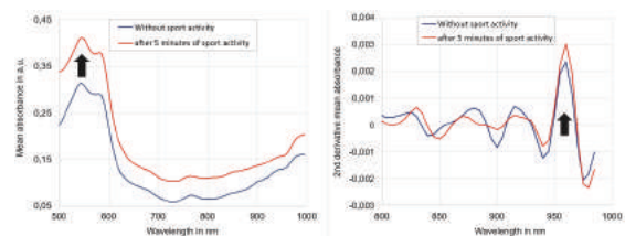
Fig. 1- Mean absorbance spectra in visual and near infrared range measured on one subject before and during sport activity (left). The largest absorbance during sport activity can be explained by an increase of tissue perfusion. The representation of the second derivative (right) shows increase of water content at 960 nm during sport activity.
