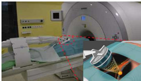
Fig. 2 - Setup of the robotic arm system in the MR-PET system in the Department of Nuclear Medicine of the University Medical Center Leipzig. The robotic arm (left) positions the US transducer according to the planned treatment. The MR-PET system monitors the position of the transducer, the temperature and the efficacy of the treatment.
