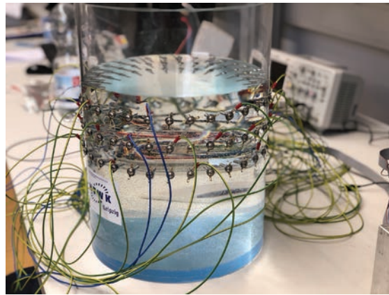
Fig. 1 - Image of the EIT phantom, filled with saline water.
