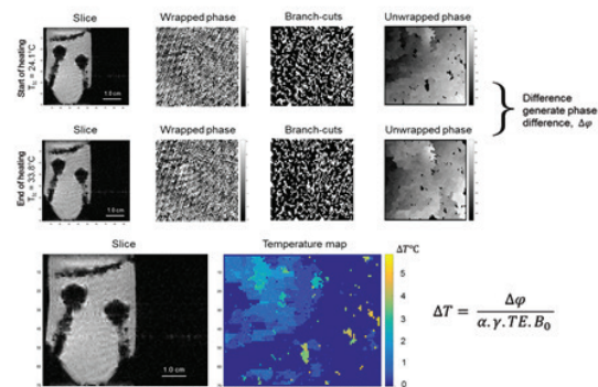
Fig. 2 - Reconstruction of MRI data to enable non-invasive temperature mapping during in vivo FUS-HT. An agar-milk phantom with a thermocouple was placed into the rat bed of the 7 T Bruker MRI with a water heating pad. Reconstruction steps of phase images for temperature mapping based on PRF thermometry.
