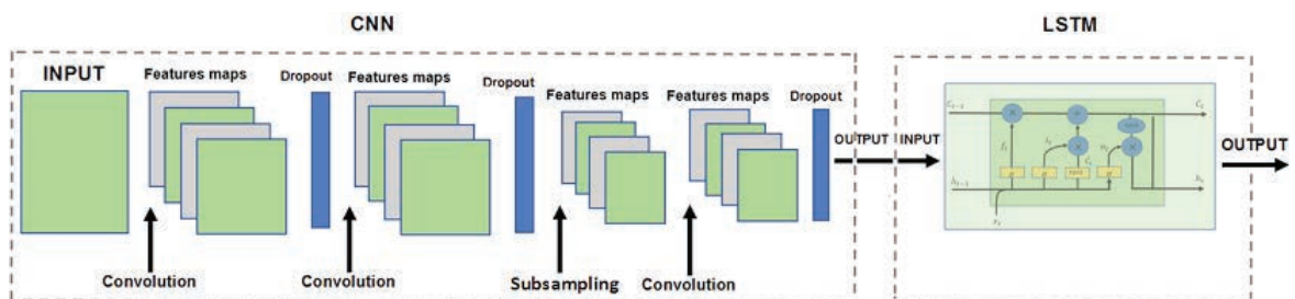
Fig. 2 - Architecture implemented.
