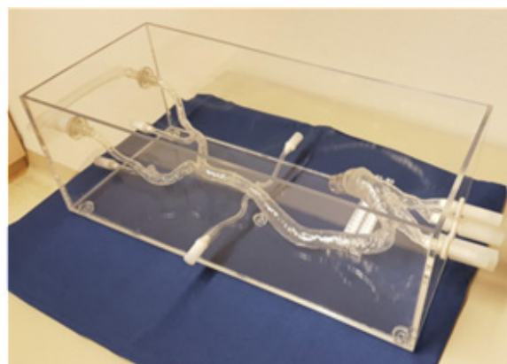
Fig. 1 - Left: 3D model of the phantom. Right: life size silicone phantom (55x25x20cm) by Phacon GmbH. A replaceable fresh porcine heart can be integrated into the phantom, as depicted in the computer model.
